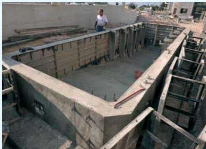
Saratoga aluminium wall forms are removed. A smooth, full 20cm thick seamless reinforced concrete pool structure is formed to last for centuries.
